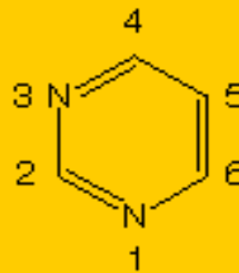
Pyrimidines
