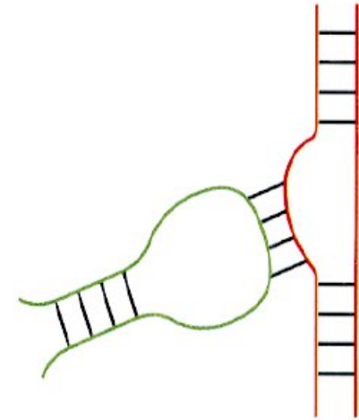
Hairpin-bulge
