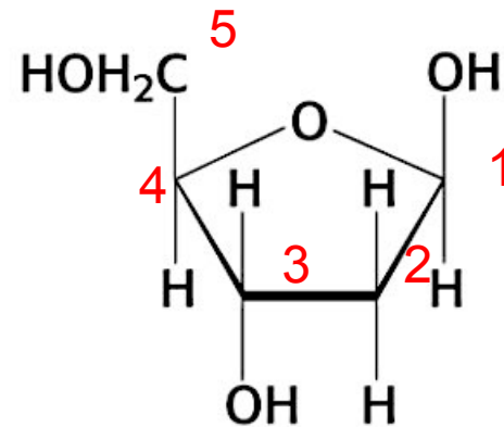
2-deoxyribose
