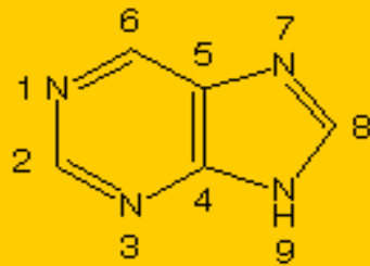
Purines
