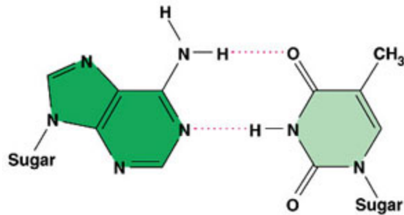
Adenine (A)
