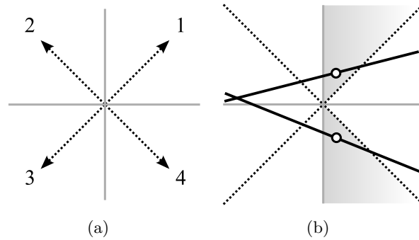
Fig. 7. (a) The asymptote spokes. (b) Subcase (3, 4, -) . The line-critical points lie in the shaded regions. If a triangle includes these two points, it must also include the origin.
