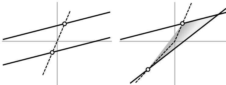
Fig. 8. Subcase (3, 4, +) . As the bottom line rotates counter-clockwise, its critical line (dashed) rotates clockwise. The triangle must contain the shaded area, and thus the origin.
