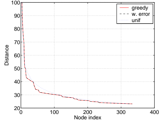
Fig. 10. Compare the deployment of the greedy algorithm with and without estimation errors.
