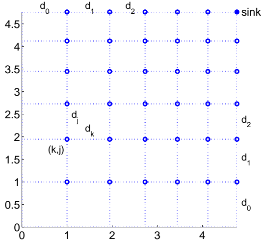
Fig. 11. Square-shape 2D deployment with total energy constraints.
