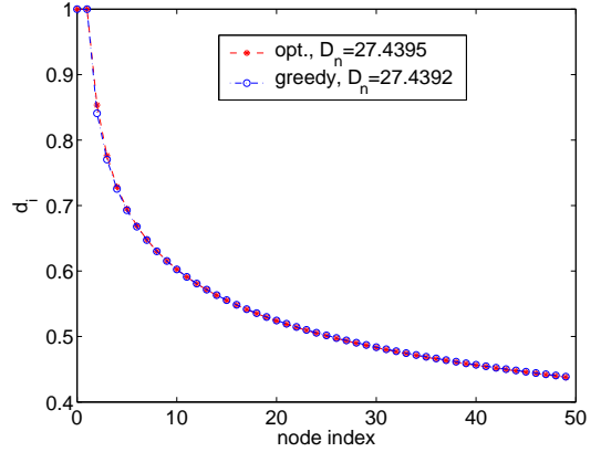
Fig. 3. Compare the locations of data back-haul nodes in the greedy scheme with the numerical solution of Problem IDEAL.
