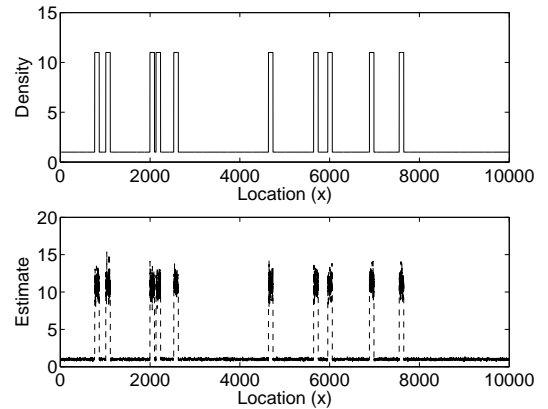
Fig. 8. Bursty data density profile.
