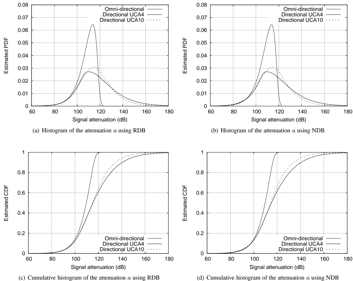
Fig. 3. Signal attenuation statistics for omnidirectional transmission, RDB, and NDB
