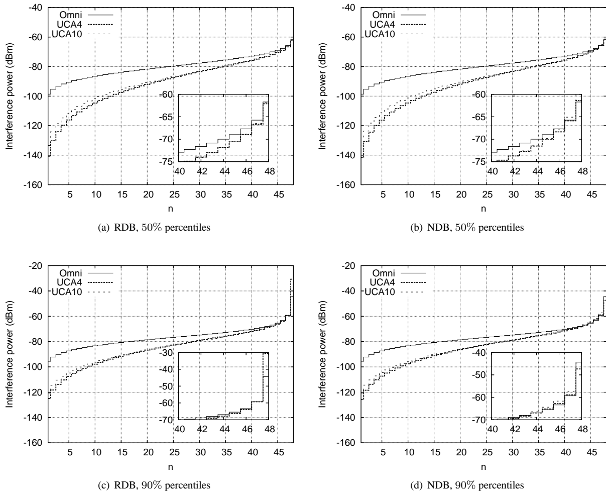
Fig. 4. Interference power at a receiving node caused by the n least interfering nodes, for the two scenarios of Fig. 3.
