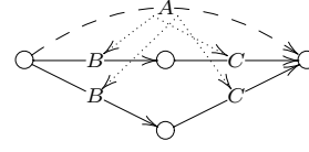
Figure 4. CFL-reachability.
