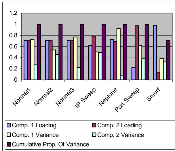
Figure 1: Component Loading and Variance
