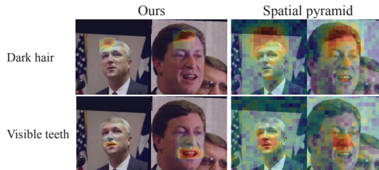
Figure 6. Spatial extent of attributes discovered by our approach vs. a spatial pyramid baseline. Red/blue indicates strong/weak attribute relevance. Spatial pyramid uses a fixed rigid grid (here 20x20), and so cannot deal with translation and scale changes of the attribute across images. Our approach is translation and scale invariant, and so its discoveries are much more precise.
