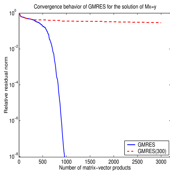
Figure 4.1: Relative residual norms of GMRES and GMRES(300).
