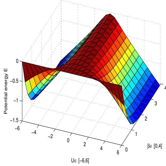
Figure 1.1: Potential energy E for t = 0, \mu = 0
