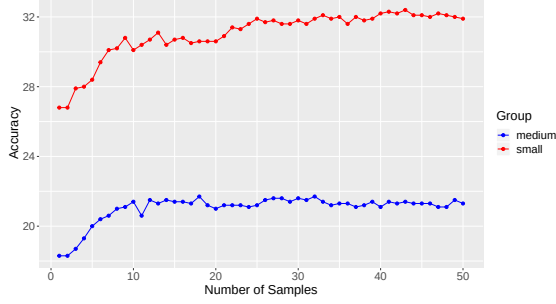
Fig. 2. Number of \mathcal{S}\text{-}\mathcal{C} samples vs. Accuracy
