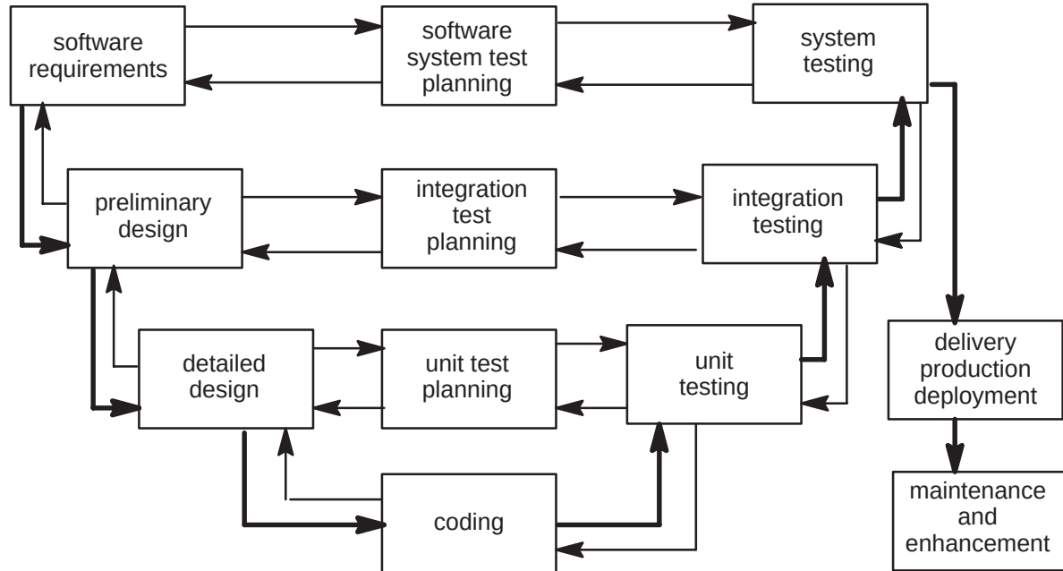
Figure 1. Software Life Cycle
