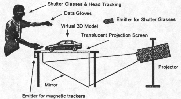
Figure 1: Hardware setup.
