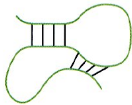
Pseudoknot
