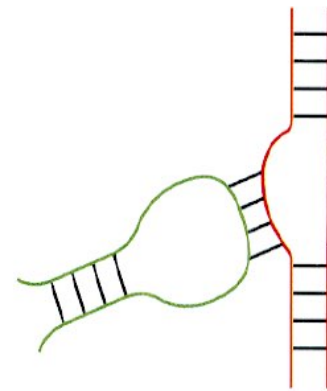
Hairpin-bulge
