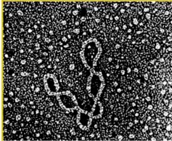
(a) Supercoiled
