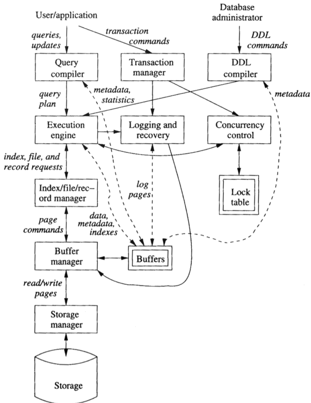
Figure 1.1: Database management system components
