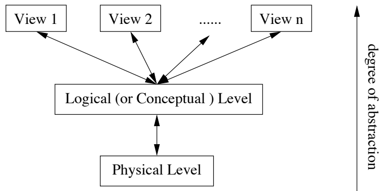
Levels of Abstraction in a DBMS
