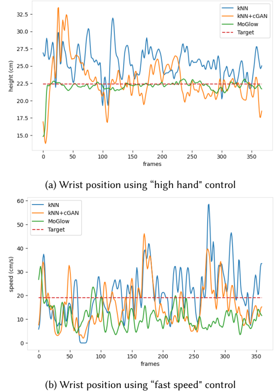
Fig. 2. Control-based comparison of left hand height (a) and velocity (b) between k-NN (ours, blue), k-NN+cGAN (ours, orange), and MoGlow ([Alexanderson et al. 2020], green) over a test sequence. The larger variation produced by our methods lead to more natural motion variations, unlike MoGlow, which could lead to a temporally static gesture w.r.t. the control signal.
