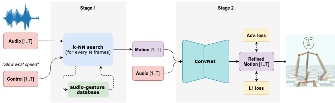
Fig. 1. Our proposed pipeline consists of two main stages. In Stage 1, we first employ a k-Nearest Neighbor search to find the most plausible sequence considering the audio and previous pose similarity in the database. At any given time step, additional information can be provided to incorporate further control over of the synthesis output. The 3D gesture generated through Stage 1 is then passed to a conditional GAN trained to produce a refined gesture sequence by comparing the output against real audio-gesture sequences.
