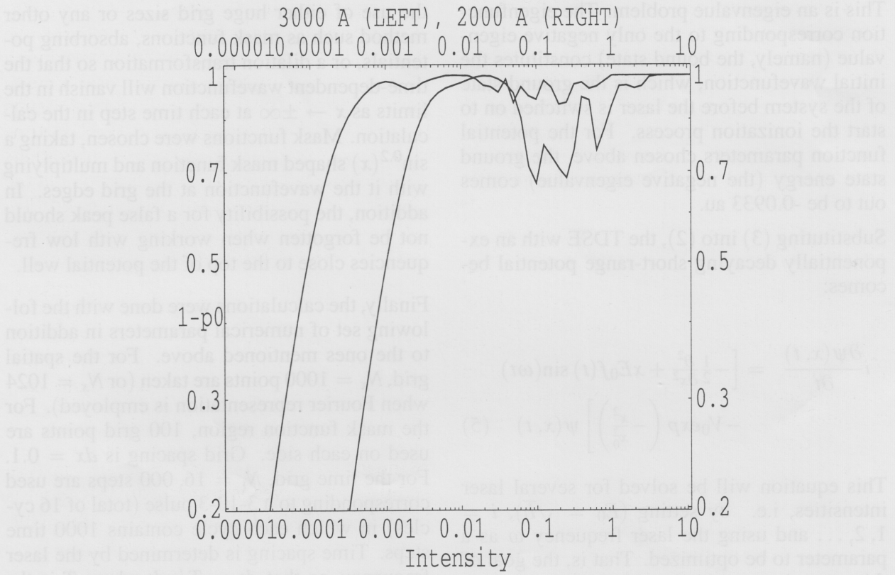
Fig. 1. End of pulse ionization 1-p_0 as a function of laser intensity, for two different frequencies. The 16-cycle pulse that was used consists of a 3-cycle smooth (sine-squared ramp) turn-on, a 3-cycle smooth turn-off and 10-cycle constant laser field inbetween. Ionization suppression at high intensities is evident in both cases. Note that for the left curve, which corresponds to \omega = 0.152 ( \lambda = 3000\text{\AA} ), the grid walls start interfering in the calculation producing a slight minimum in the structure around I = 0.001 . This frequency is a 1-photon promotion from the ground state to slightly above the top of the well. The minimum will sharpen as the frequency is lowered. For higher frequencies, no minimum appears but the curve is shifting to the right, towards the higher intensity region. The right curve corresponds to a frequency of \omega = 0.228 ( \lambda = 2000\text{\AA} ). In atomic units, I = 1.0 corresponds to I = 3.5 \times 10^{16} \text{ W/cm}^2 .
