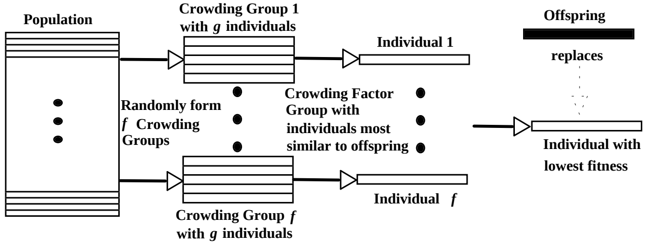
Figure 1: Worst among most similar (WAMS) replacement policy
