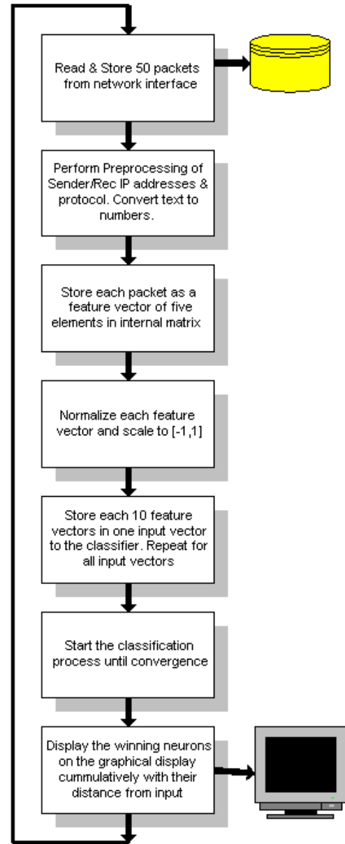
Figure 1: Block Diagram of NSOM
